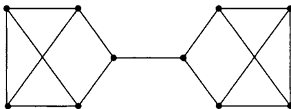
FIGURE IX.3. A cubic graph of order 10 and conductance 1/15 .
