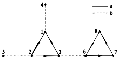
FIGURE VIII.2. Construction of a Cayley diagram.
