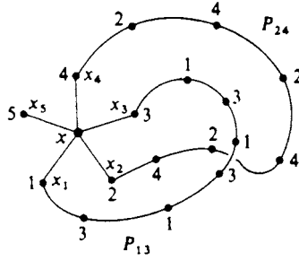
FIGURE V.4. The paths P_{13} and P_{24} .
