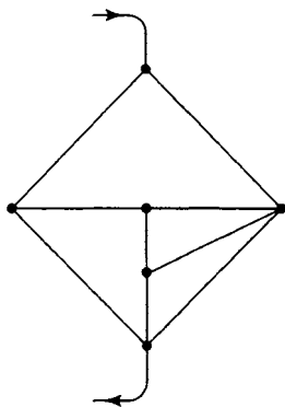
FIGURE II.17. A plane network.
